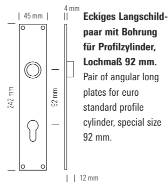
Eckiges Langschildpaar blind. Pair of angular long plates blind.
